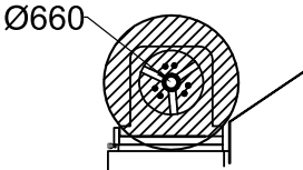
SWING OVER BED
