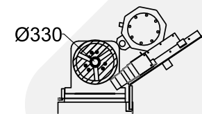
SWING OVER CARRIAGE
