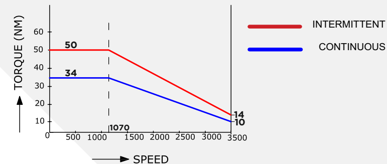
SPINDLE TORQUE V/S SPEED
