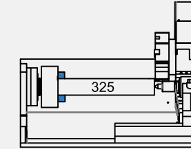
MAX TURNING LENGTH
