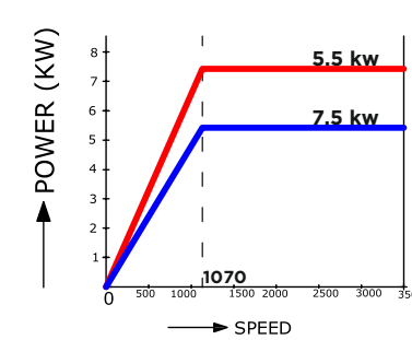
SPINDLE POWER V/S SPEED
