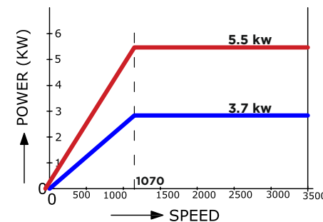
SPINDLE POWER V/S SPEED
