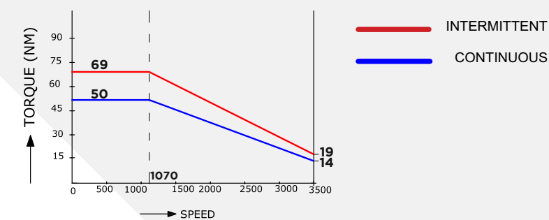
SPINDLE TORQUE V/S SPEED
