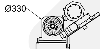
SWING OVER CARRIAGE
