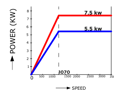
SPINDLE POWER V/S SPEED
