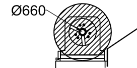
SWING OVER BED
