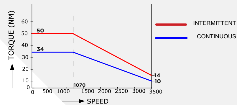
SPINDLE TORQUE V/S SPEED
