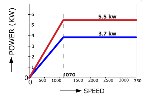
SPINDLE POWER V/S SPEED
