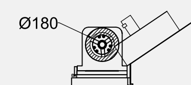
MAXIMUM TURNING DIA
